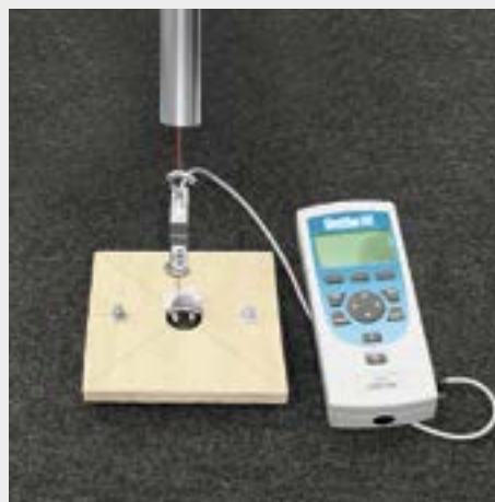
Testing of fixing element strength
